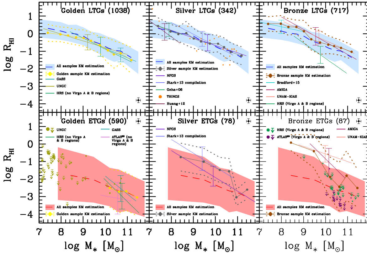
Fig. 3. Atomic gas-to-stellar mass ratio as a function of M_* for the Golden, Bronze, and Silver LTGs (upper panels) and ETGs (lower panels). The mean and standard deviation in different mass bins, taking into account upper limits by means of the Kaplan-Meier estimator, are plotted for each case (filled circles connected by a dotted line and dotted lines around, respectively). For comparison, the mean and standard deviation (dashed lines and shaded area) from all the LTG (ETG) samples are reproduced in the corresponding upper (lower) panels. For each sample compiled and homogenized from the literature, the Buckley-James linear regression is applied, taking into account upper limits. The lines show the result, covering the range of the given sample; the error bars show the corresponding standard deviations obtained from the regression. When the data are too scarce and dominated by upper limits, the linear regression is not applied but the data are plotted. The numbers of LTG and ETG objects in each category are indicated in the respective panel. The color figure can be viewed online.
