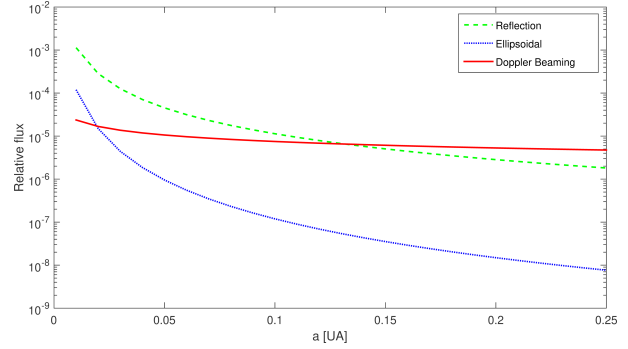
Fig. 1. Small scale photometric variations of a phase curve as a function of the radial semi-major axis of the planet orbit. The color figure can be viewed online.
