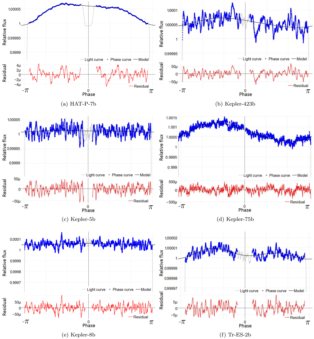
Fig. 4. Light curve, phase curve, fit model, and residual for the different planets we found with coherent effect sign. The color figure can be viewed online.
