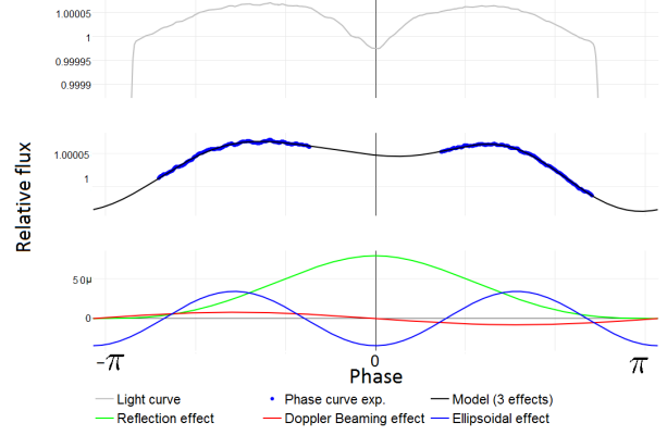
Fig. 2. KOI-13b phase curve fitting. The color figure can be viewed online.
