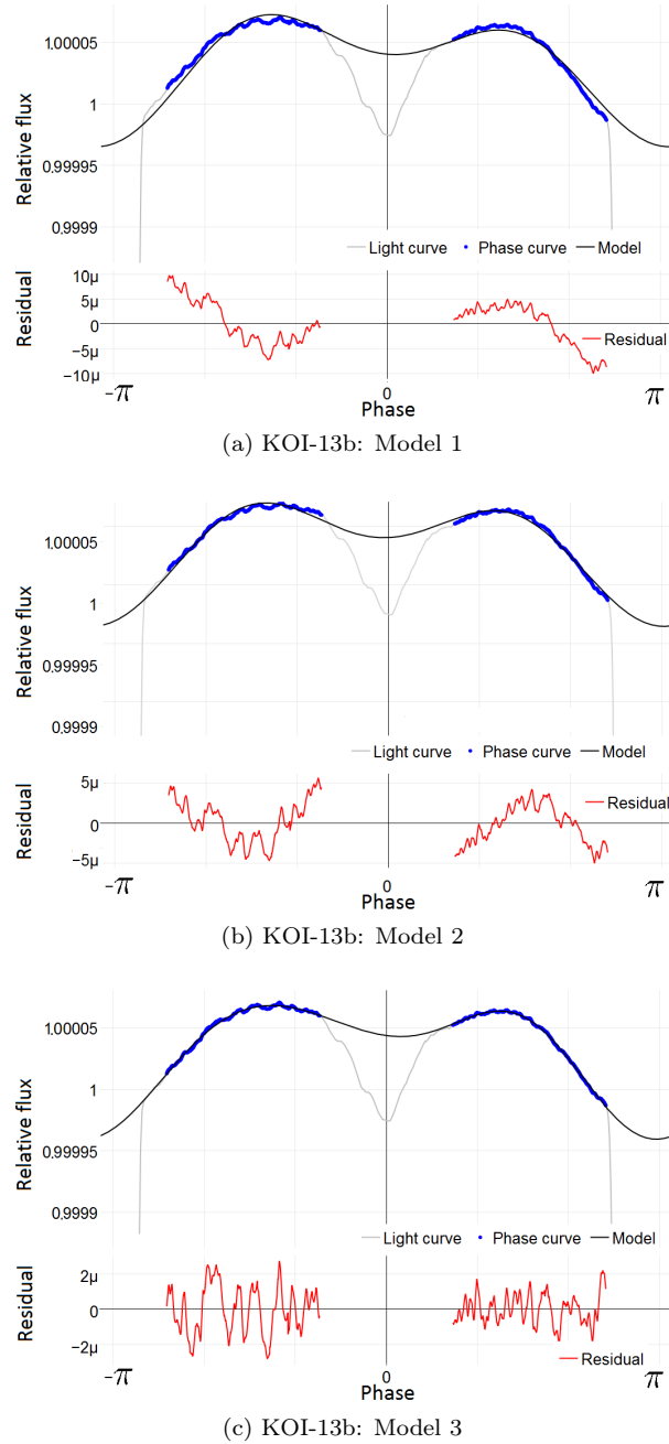
Fig. 3. KOI-13b planetary light curve, phase curve, fitting model, and residuals for each of the three models indicated in the text. The color figure can be viewed online.
