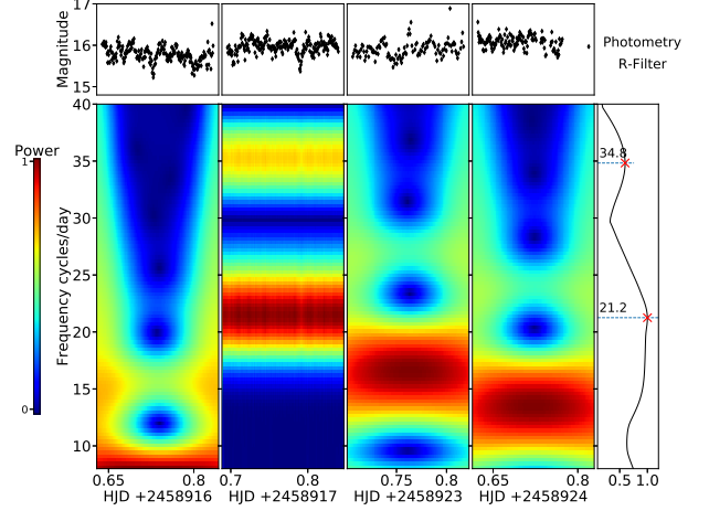
Fig. 15. Scalogram of the R-band photometric data. The global spectrum is exhibited in the utmost right panel, while the local spectrum appears in the panels below the data of each night. The second night shows the presence of the spin period and a \approx 21 cycles/day signal (consistent with the spin-orbit beat period). The rest of the nights are dominated by the orbital cycle. See text for further discussion. The colour figure can be viewed online.
