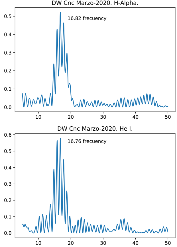
Fig. 8. Top: Power spectra of H \alpha using GAU2. Bottom: Power spectra of the He I \lambda 5876 Å emission line using GAU2. See text for further discussion. The colour figure can be viewed online.
