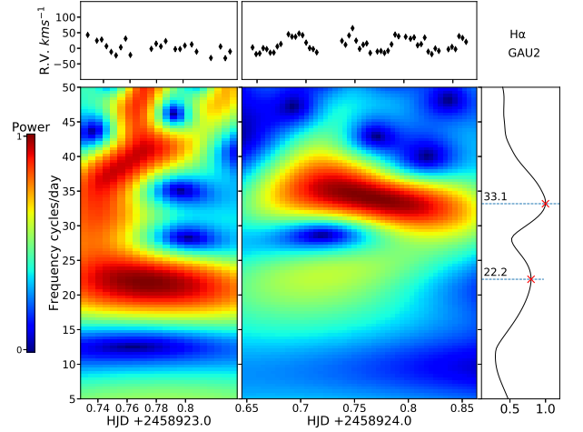
Fig. 16. Scalogram of the H \alpha GAU2 spectroscopic data. The global spectrum is exhibited in the utmost right panel, while the local spectrum appears in the panels below the data of each night. The first night shows prominent signals at \approx 37 cycles/day and \approx 22 cycles/day. The latter signal also appears during the second night but is surpassed in intensity by a \approx 33 cycles/day signature. See text for further discussion. The colour figure can be viewed online.
