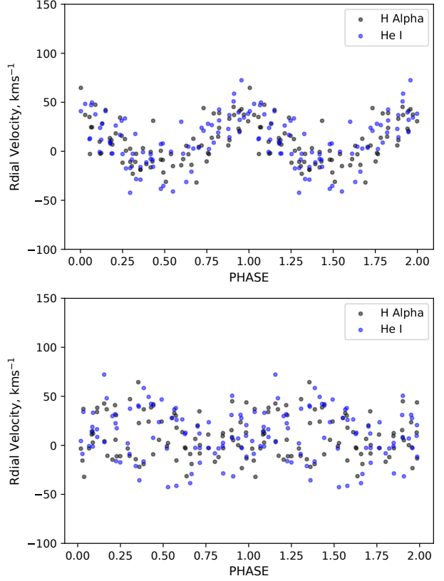
Fig. 10. Folded spectroscopic data. The top panel is folded by the orbital period. The bottom panel is folded by the spin period. The colour figure can be viewed online.
