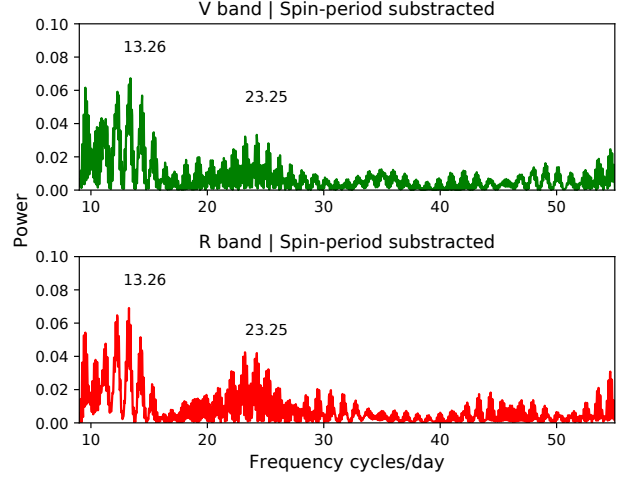
Fig. 6. Power spectrum of the residuals, after removing the spin period signal from the photometric data. The colour figure can be viewed online.
