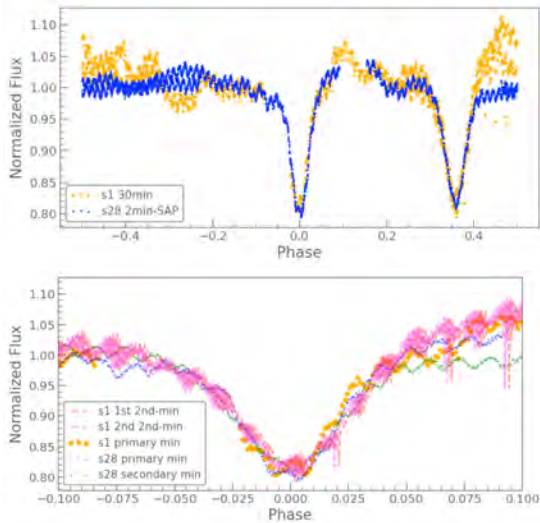
Fig. 21. Normalized TESS photometric data for Sectors 1 and 28 (s1, s28) showing the primary eclipse at phase = 0 and on top of the light curve folded with the period P = 19.2654 d. Clearly seen are the oscillations with a period of P_{\text{osc}} = 0.25 d, observed at both eclipses of the Star A + Star B system. Upper panel: Two secondary and one primary eclipse were observed in Sector 1 and one primary and one secondary were observed in Sector 28. Lower panel: As above, but the abscissa gives the distance in orbital phase from mid-eclipse of the five eclipses. The color figure can be viewed online.
