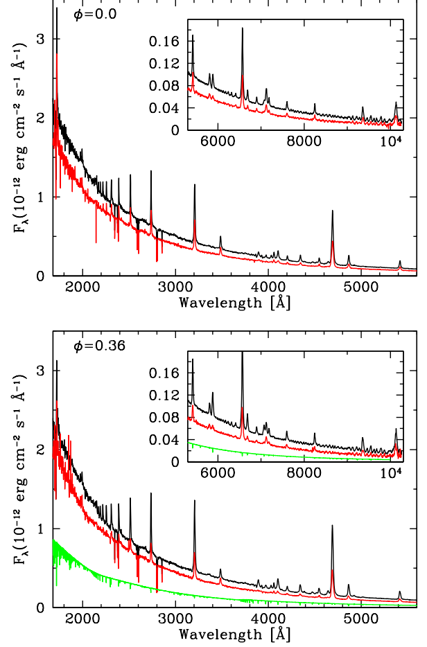
Fig. 2. Spectral energy distribution in epochs 1999-2000 (black) and 2014-2016 (red) obtained with HST/STIS showing the changes between the high (black) and low states (red) states. The top panel shows spectra at orbital phase \phi=0 and the bottom panel at \phi=0.36 . The green spectrum in the bottom panel is a CMFGEN model of Star C . The color figure can be viewed online.
