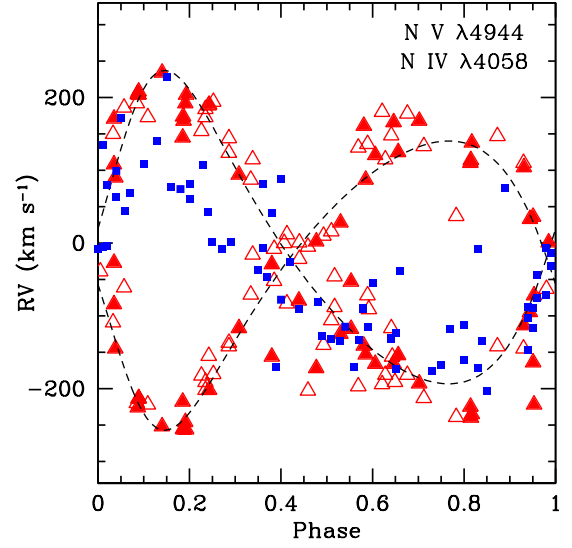
Fig. 5. Radial velocity of NV \lambda 4944 as a function of orbital phase for epochs 2008-2012 (filled triangles) and 2013-2020 (open triangles), and N IV \lambda 4058 (filled squares). The dash curves indicate the orbital solution given in Koenigsberger et al. (2014). The velocities are corrected for the SMC velocity. The color figure can be viewed online.
