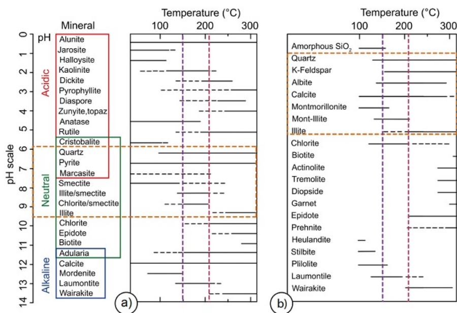
FIGURE 18 Thermal stability of various hydrothermal minerals (modified after Hedenquist et al., 2000 and Henley and Ellis, 1983). (a) Mineral assemblages associated to pH and temperature; (b) Mineral assemblages associated only to temperature. Dashed orange lines indicate the pH and estimated temperature values prevailing in the hot spring waters reported this study (purple and red dashed lines correspond to minimum and maximum estimates respectively).
