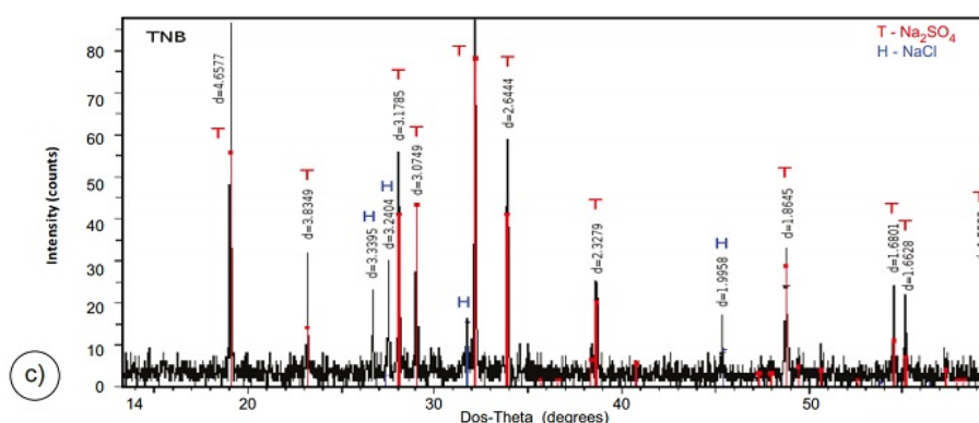
FIGURE 10 (CONT.) XRD diffractograms of precipitated salt samples collected at the (a) CMP, (b) TCH and (c) TNB hot springs.
