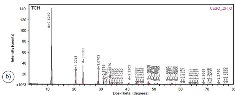
FIGURE 10 (CONT.) XRD diffractograms of precipitated salt samples collected at the (a) CMP, (b) TCH and (c) TNB hot springs.
