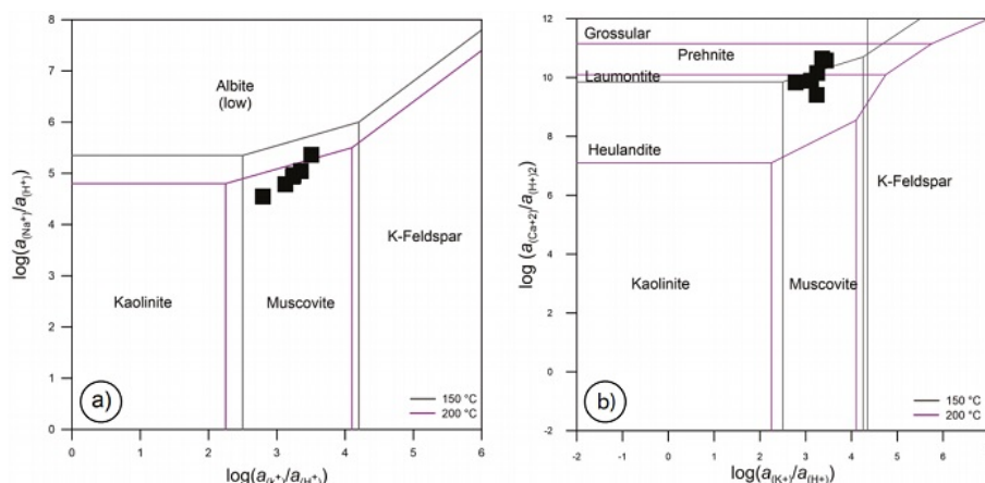
FIGURE 17 Fluid-mineral stability diagrams obtained for the (a) \text{Na}_2\text{O-K}_2\text{O-Al}_2\text{O}_3\text{-SiO}_2\text{-H}_2\text{O} and (b) \text{CaO-K}_2\text{O-Al}_2\text{O}_3\text{-SiO}_2\text{-H}_2\text{O} systems.
