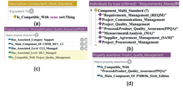
Fig. 10. (a) Definition of the class Component_Multi_Standard ; (b) Inference of instances of the class Component_Multi_Standard ; (c) Example of Component_Multi_Standard ; (d) Example of Component_Multi_Standard
