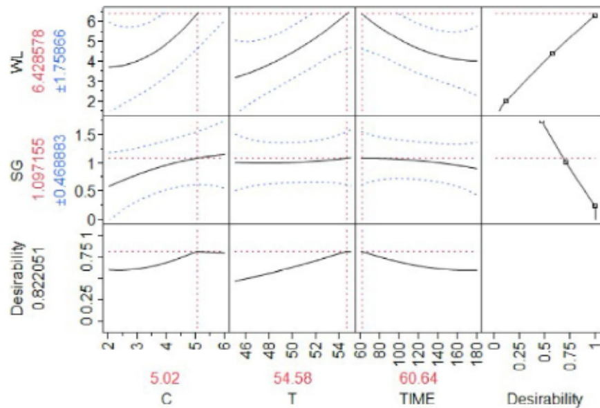
Fig. 5: Prediction profiler for optimized conditions
