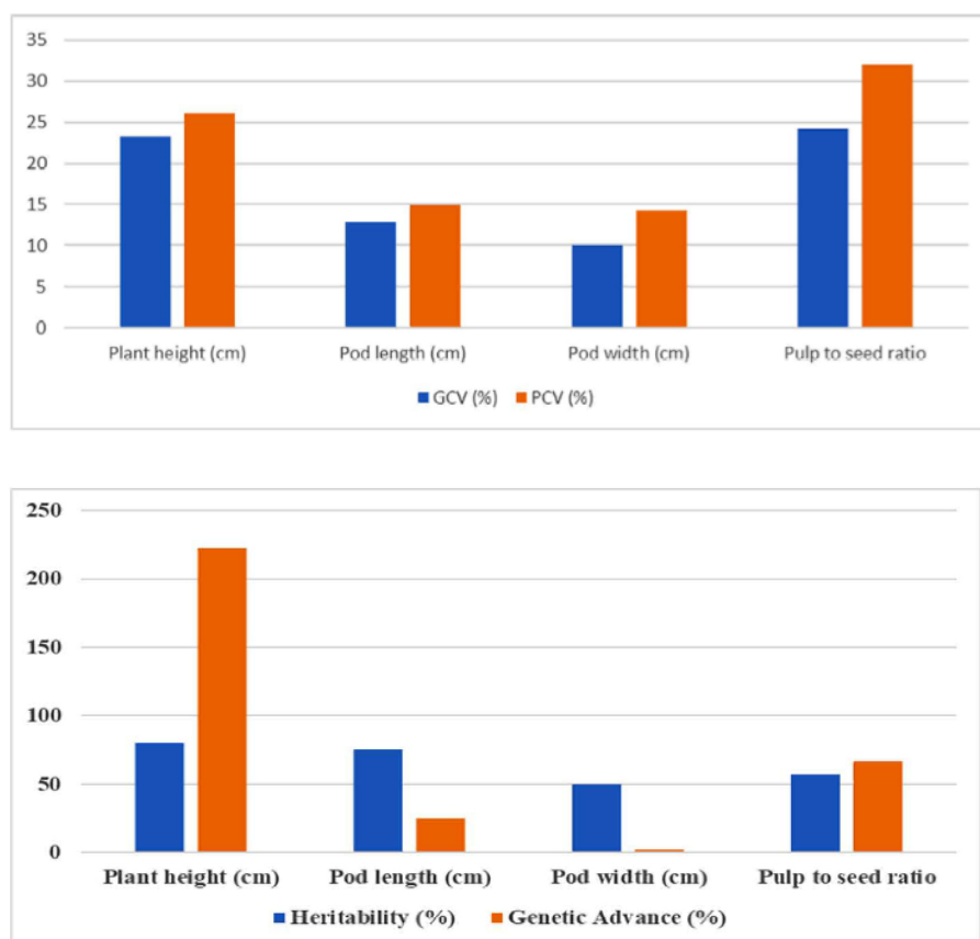
Fig. 2 Heritability and genetic advance for yield attributing traits in M2 generation
