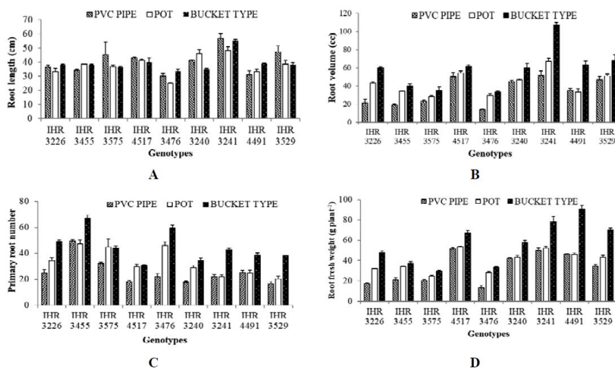
Figure 1 Influence of containers on root length (A), root volume (B), primary root number (C) and root fresh weight (D) of Capsicum sp.
