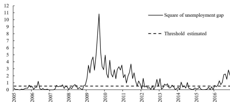
Figure 10 Variable of interest to determine the regimes: square of the traditional unemployment gap, \tau = 0.52
