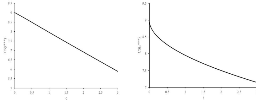
Figure 6 Comparative statics of the equilibrium social welfare
