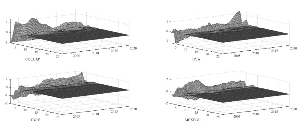
Figure 3. Impulse-response functions surfaces obtained from a USEPU shock to COLCAP, IPSA, IBOV, and MEXBOL returns
