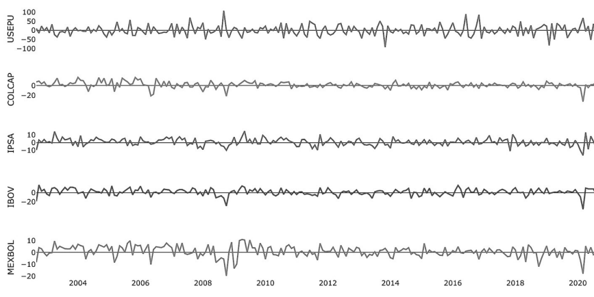
Figure 1. Logarithmic growth rates of USEPU, COLCAP, IPSA, IBOV and MEXBOL, 08/01/2002 to 8/1/2020
