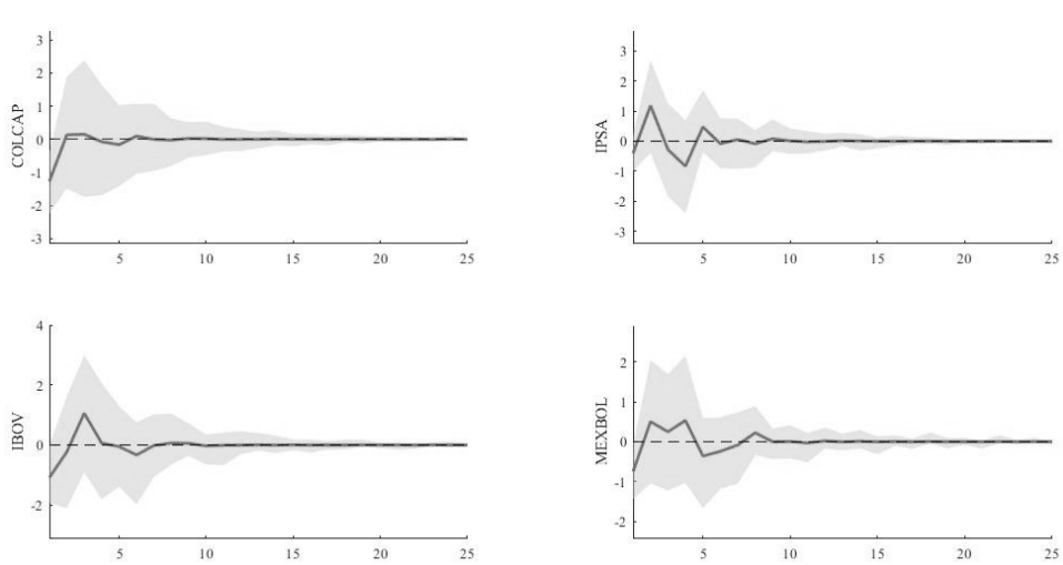
Figure 2. Impulse-response functions from a shock from the USEPU to COLCAP, IPSA, IBOV, and MEXBOL returns
