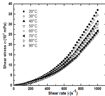
Figure 1. Whey rheograms
