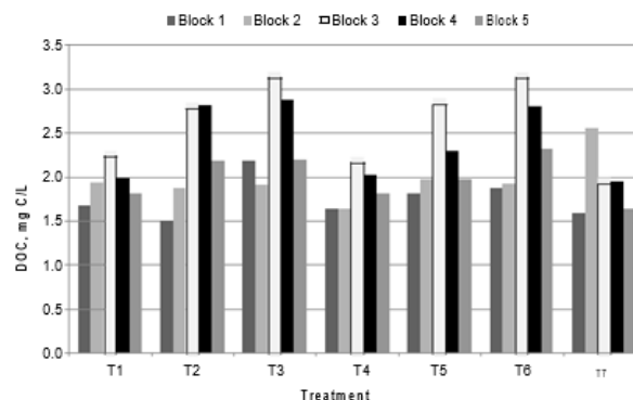
Fig. 5. DOC of the water clarified in treatments
