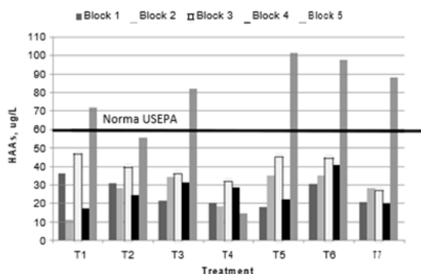
Fig. 10. HAAs generated in treatments
