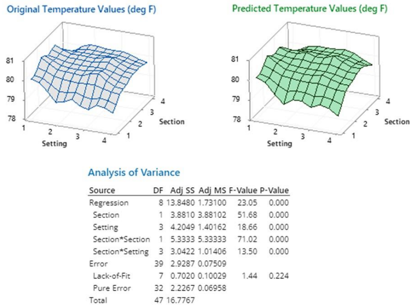
Fig. 7. Statistical modeling and analysis of variance (low p-values in the last column indicate significant effects of the sources of variation in the first column).
