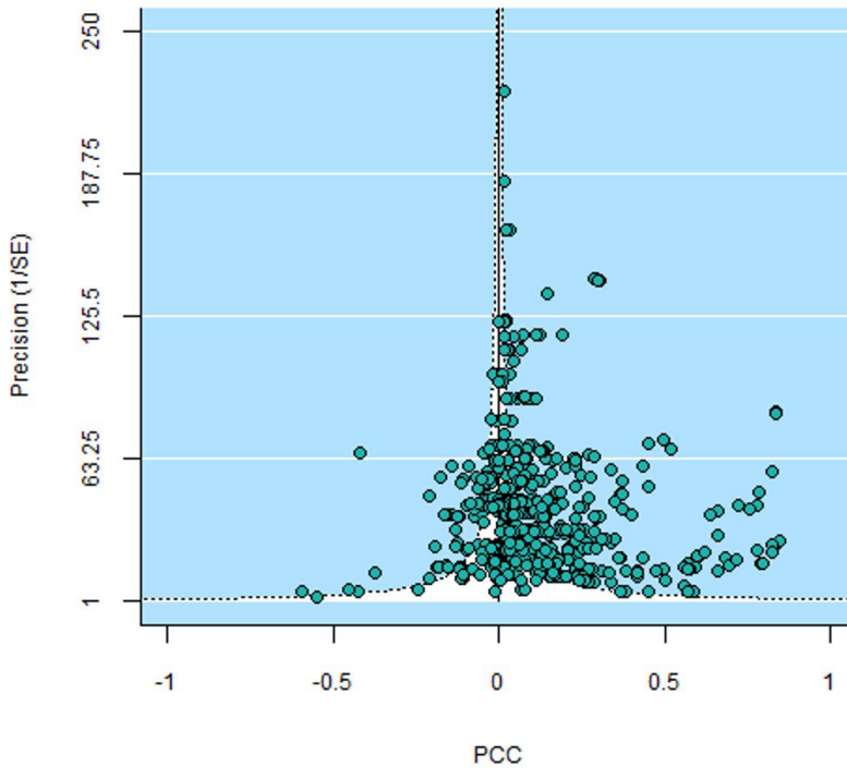
FIGURE 3 PCC funnel plot.
