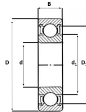
Figure 2. Sectional drawing of bearing.
