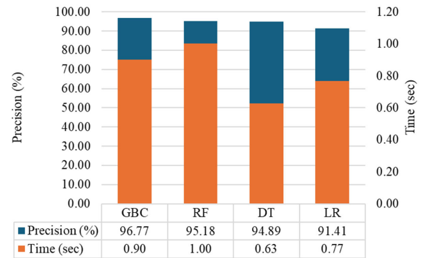
Figure 2. Accuracy and execution time of the top-rated automatic learning algorithms
