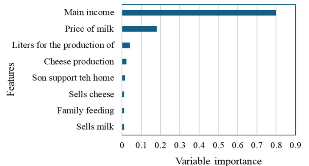
Figure 3. Important features of the GBC model
