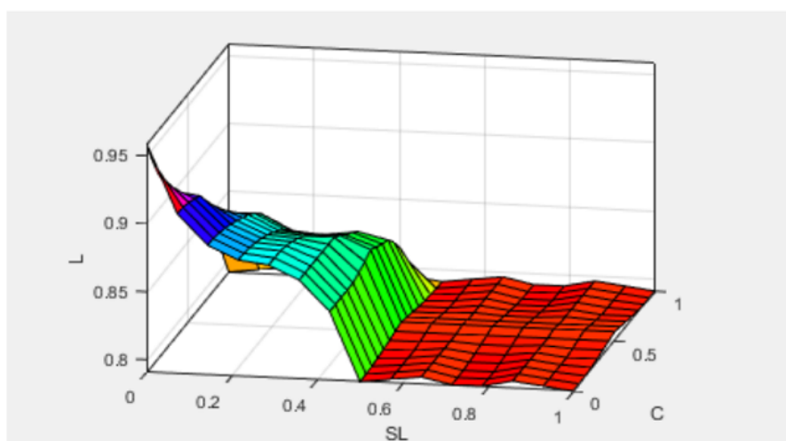
FIGURE 7 3D Plot of the fuzzy output of smart street lighting
