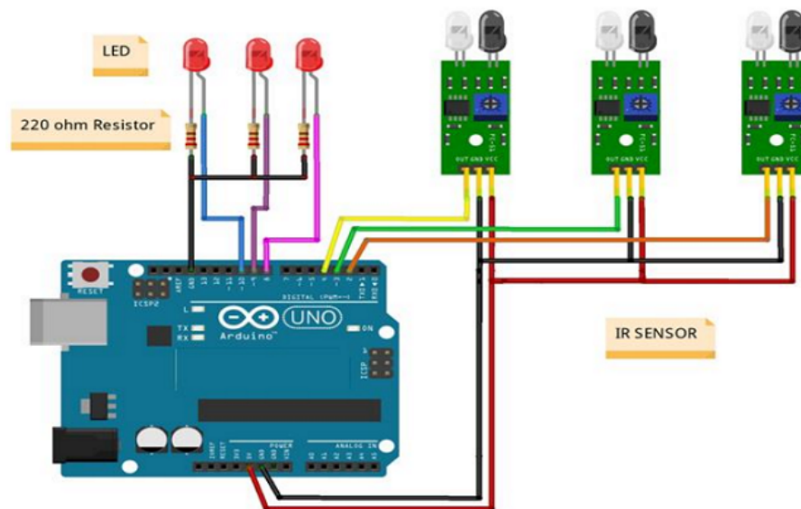
FIGURE 1 Design of a street lighting system
