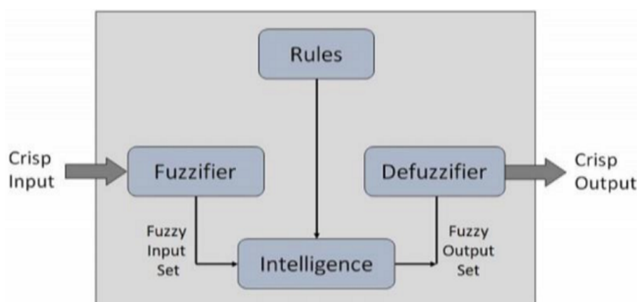
FIGURE 3 Fuzzy logic
