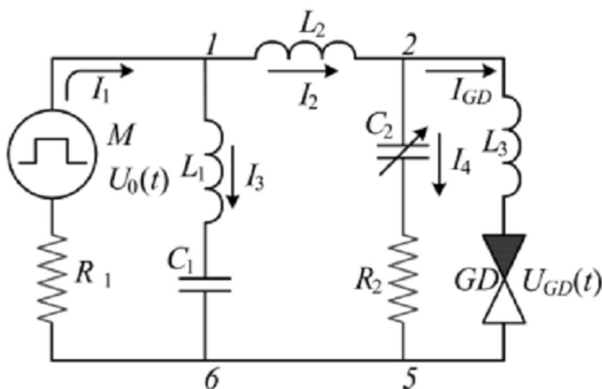
FIGURE 2 Equivalent circuit simulating a Gunn oscillator in a resonator
