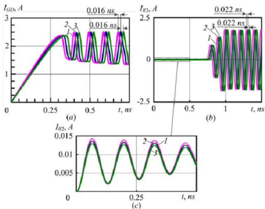
FIGURE 3 Time dependences of the Gunn diode current at voltage pulse rise times t_c of 0.95 (1), 1 (2), and 1.05 ns (3) for the single-layer structure (a) in the circuit with resistive load and (b) at the load R_2 in the equivalent circuit, U_0 = 20 V.
