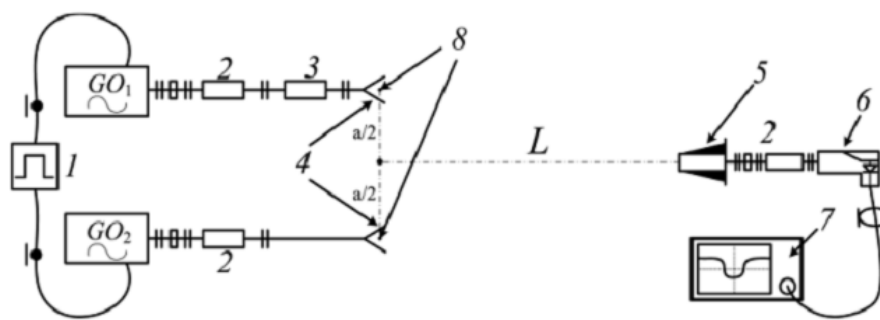
FIGURE 8 Experimental setup of a wave field measurement of an antenna system
