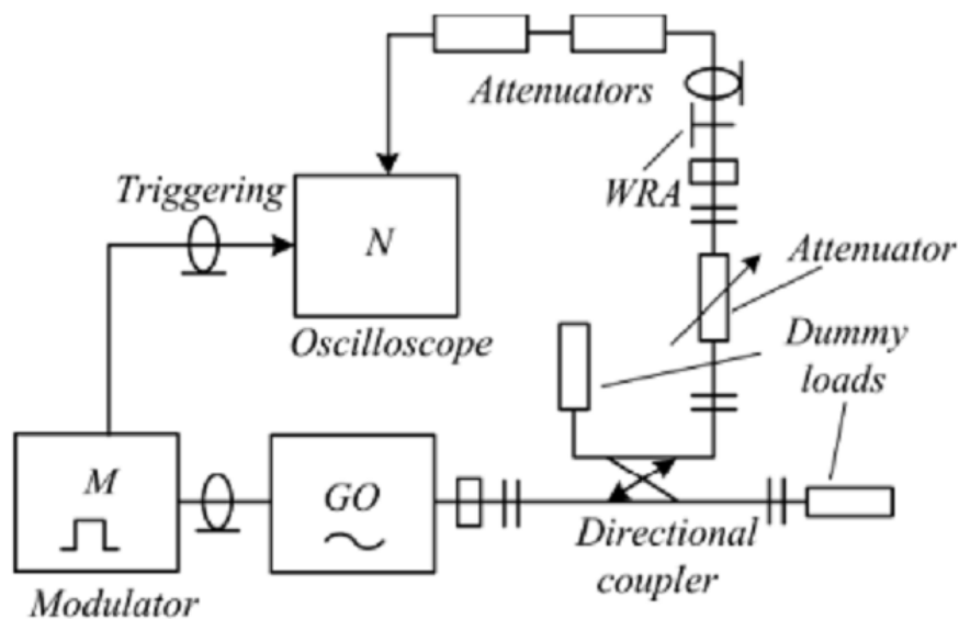
FIGURE 4 Measuring circuit for the standard deviation of phase delay
