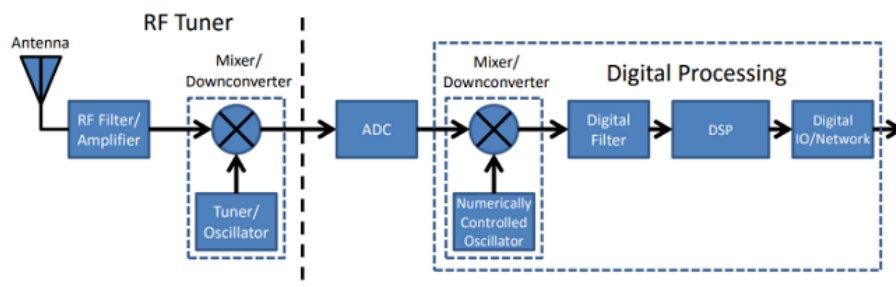
FIGURE 1 SDR Receiver (Benks, 2016)
