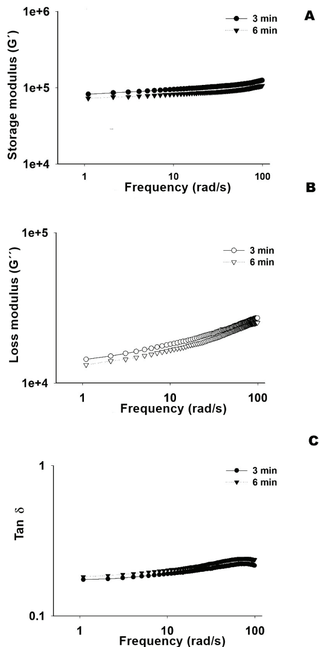
Figure 3. Effect of mixing time on viscoelasticity of the corn dough. A, storage moduli, G' ; B, loss moduli G'' ; C, phase angle \tan \delta as a function of frequency.
