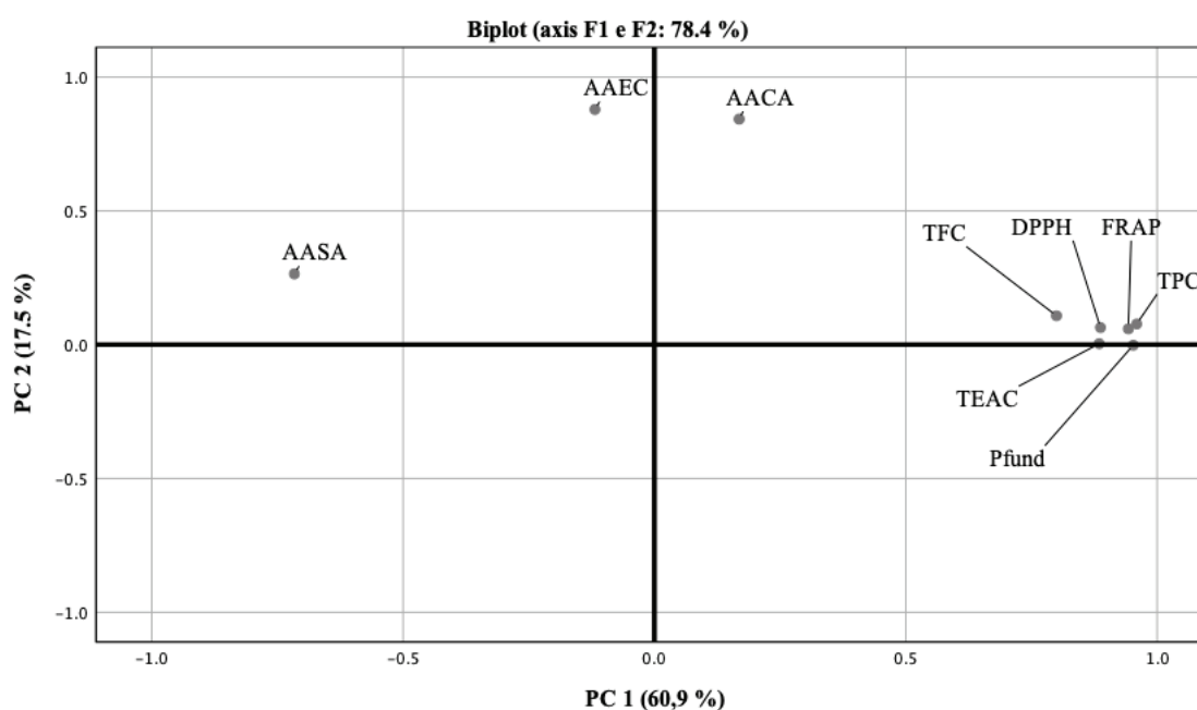
Figure 2. Principal component analysis plot of the evaluated parameters.
