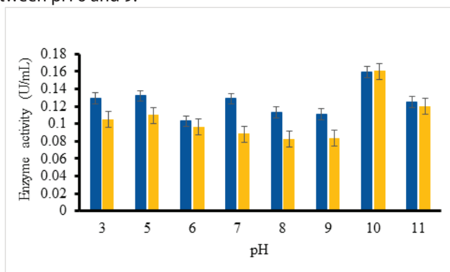
Figure 4. Effect of pH on the activity of the E. faecium E68 extracellular lipase enzyme. — Olive oil waste (U/mL), — Medium (U/mL)
