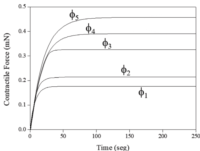
Figure 9. Generative force at pH = 2 of a single PAN fiber with different diameters: \phi_1 = 91 \mu\text{m} , \phi_2 = 102 \mu\text{m} , \phi_3 = 219 \mu\text{m} , \phi_4 = 237 \mu\text{m} and \phi_5 = 287 \mu\text{m}
