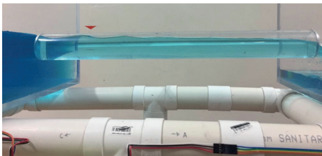
Figure 6. Undular hydraulic jump at the inlet caused by flow depression under weir-type operating.
