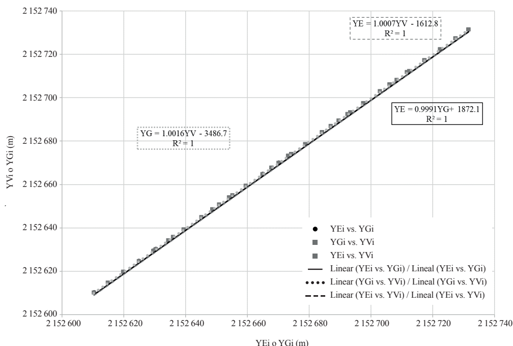
Figure 4. Comparison of Mercator Universal Transverse coordinates (UTM, from zone 14N) latitudinal (Y variables) between the three surveying methods: total station (TS; YE i ), GPS RTK (YG j ) and unmanned aerial vehicle (UAV; YV i ).
