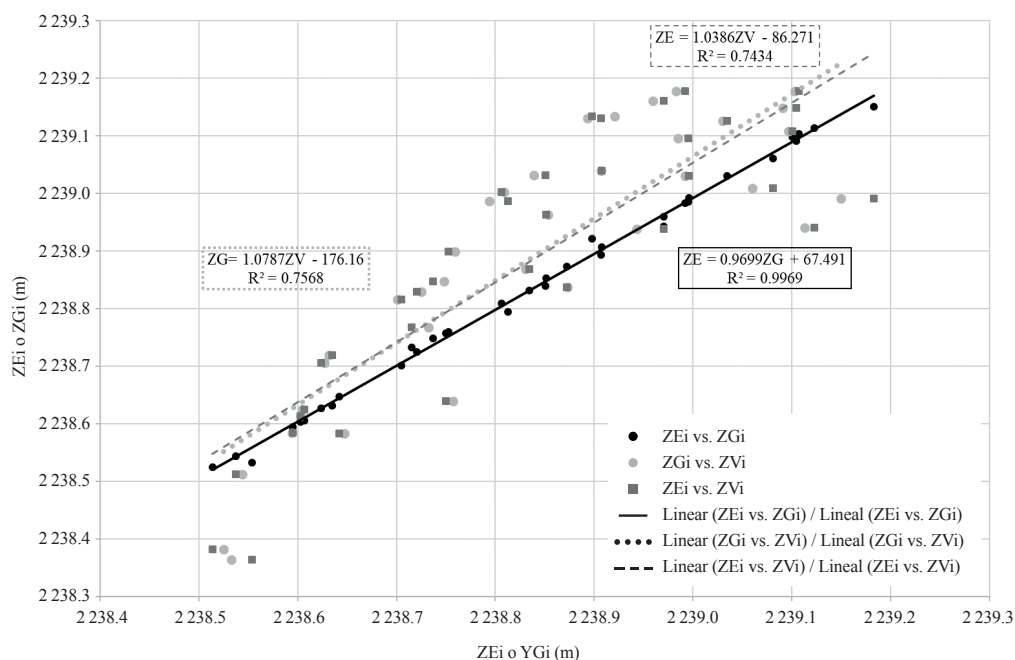
Figure 5. Comparison of Mercator Universal Transverse coordinates (UTM, from zone 14N) altitudinal (Z variables) between the three surveying methods: total station (TS; ZE i ), GPS RTK (ZG j ) and unmanned aerial vehicle (UAV; ZV i ).
