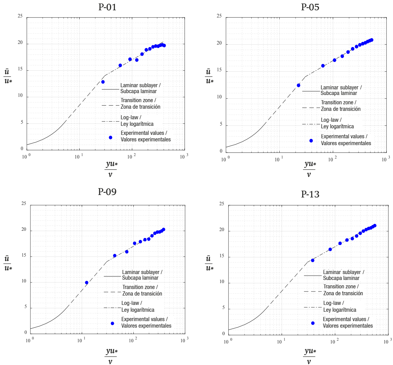
Figure 3. Dimensionless profiles of mean velocities, the von Kármán model and experimental values.
