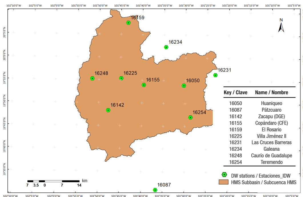
Figure 7. Weather stations used in this study.
