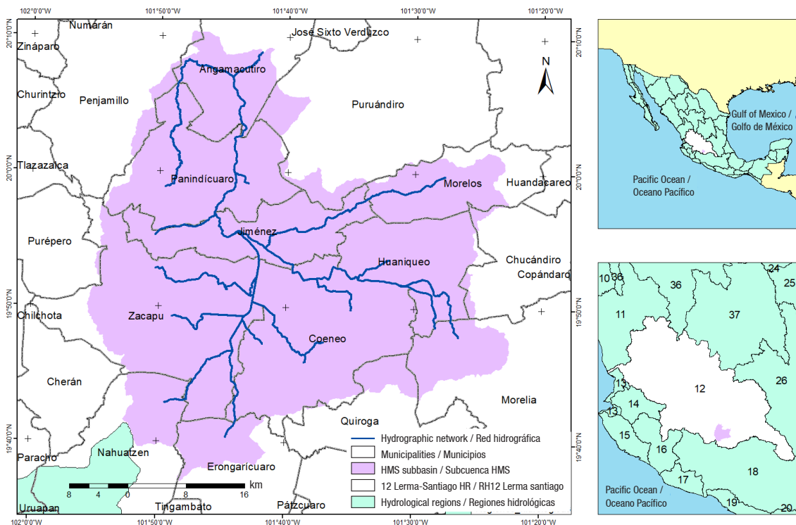
Figure 3. Location of the basin (HEC-GeoHMS).
