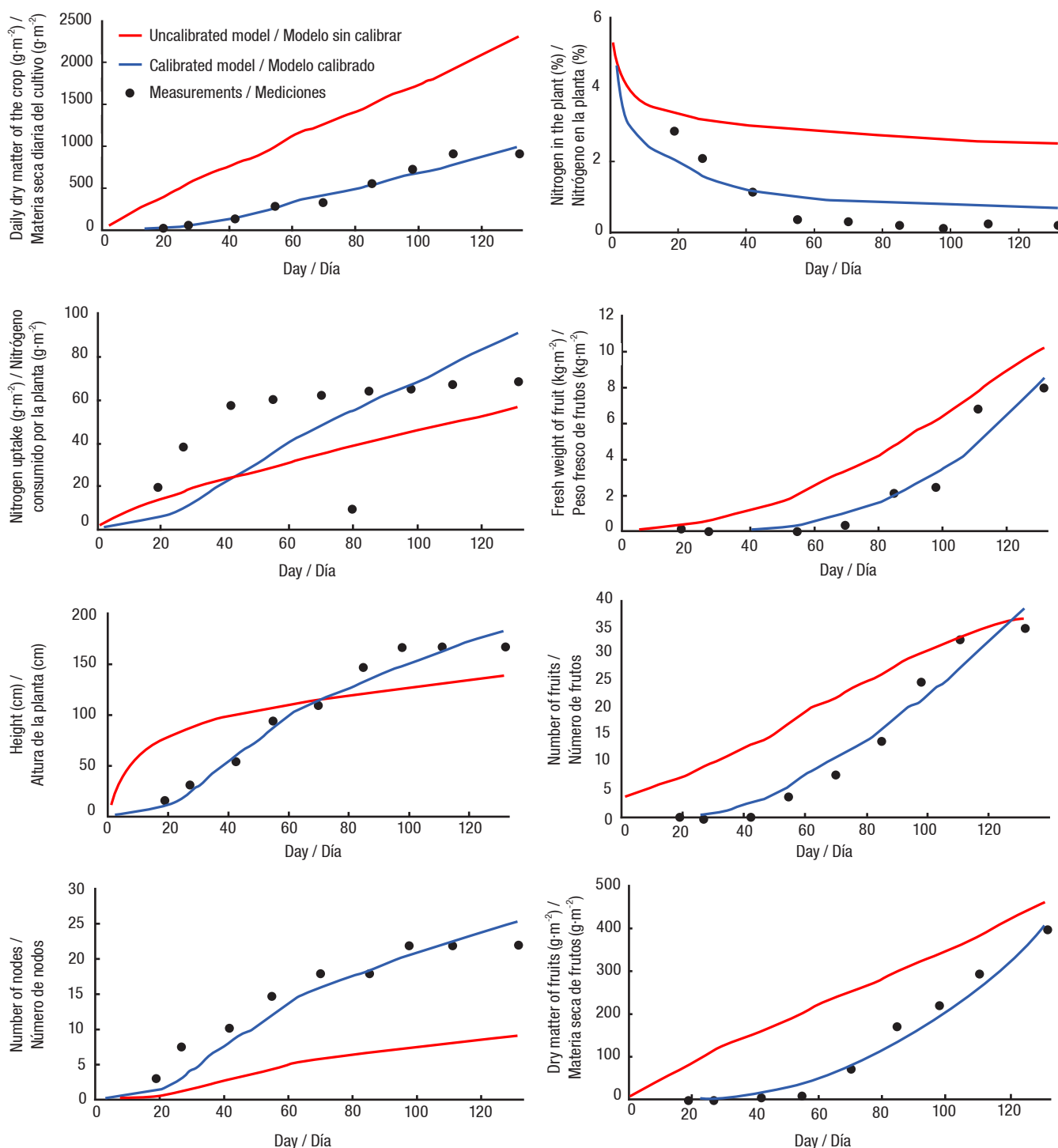
Figure 1. Behavior of the VegSys model with and without calibration for the first growing cycle.
