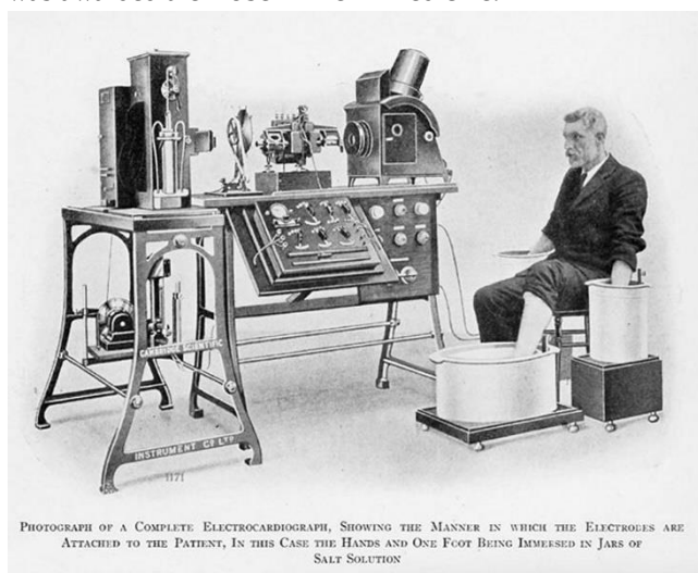
Figure 3: First table model Einthoven electrocardiogram manufactured by the Cambridge Instrument company of London in 1911. Showing the manner in which, the electrodes are attached to the patient, in this case the hands and one foot being immersed in jars of salt solution [16].
