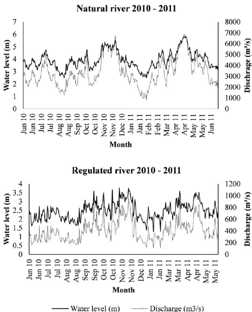
FIGURE 2. Water level (m) and discharge (m 3 /s) from June 2010 to June 2011 for natural and regulated flow rivers from the Magdalena basin.
