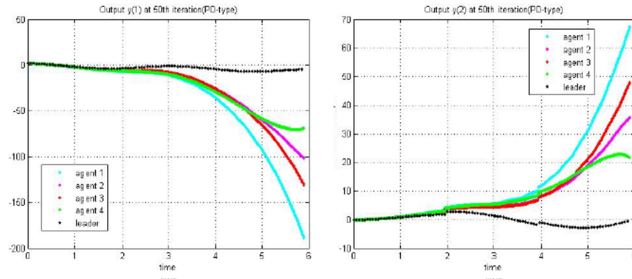
Figure 9. The trajectory of the 50th iteration (PD-type).
