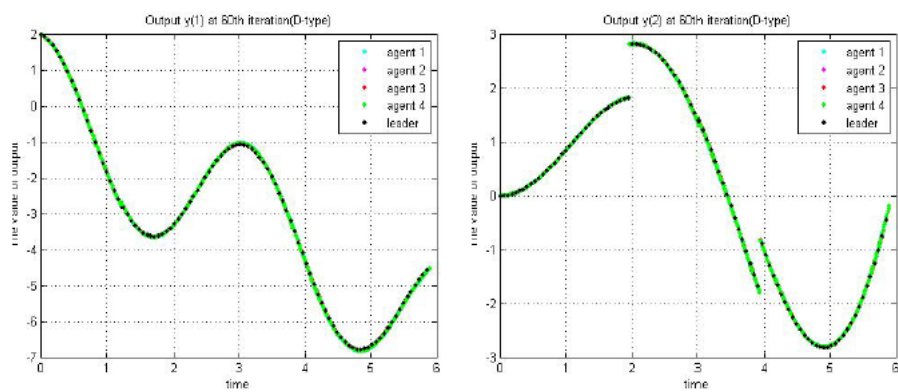
Figure 7 The trajectory of the 60th iteration (D-type).
