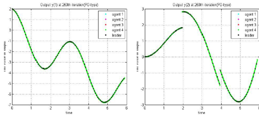
Figure 11. The trajectory of the 250th iteration (PD-type).
