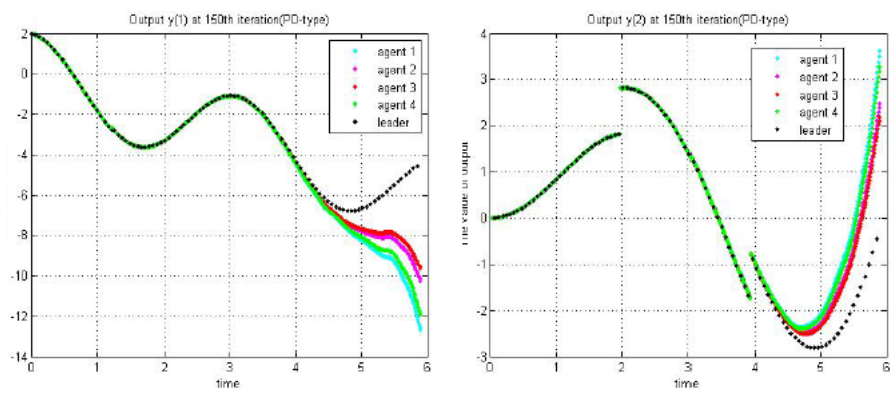
Figure 10. The trajectory of the 150th iteration (PD-type).
