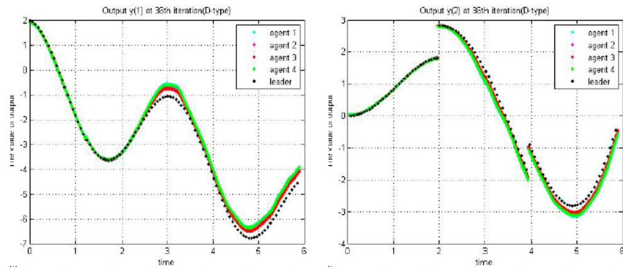
Figure 6. The trajectory of the 36th iteration (D-type).
