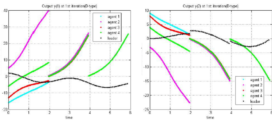
Figure 4. The trajectory of the first iteration (D-type).
