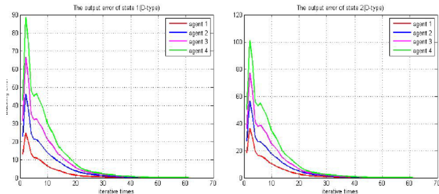
Figure 2. The output error (D-type)
