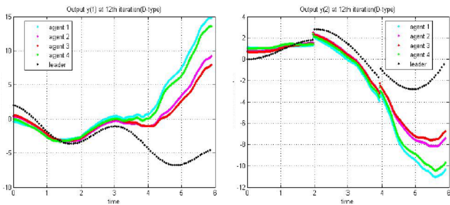
Figure 5. The trajectory of the 12th iteration (D-type).
