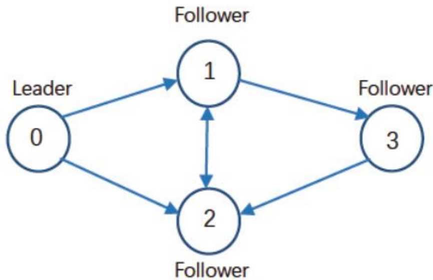
Figure 1. The communication topology of multiagent systems.
