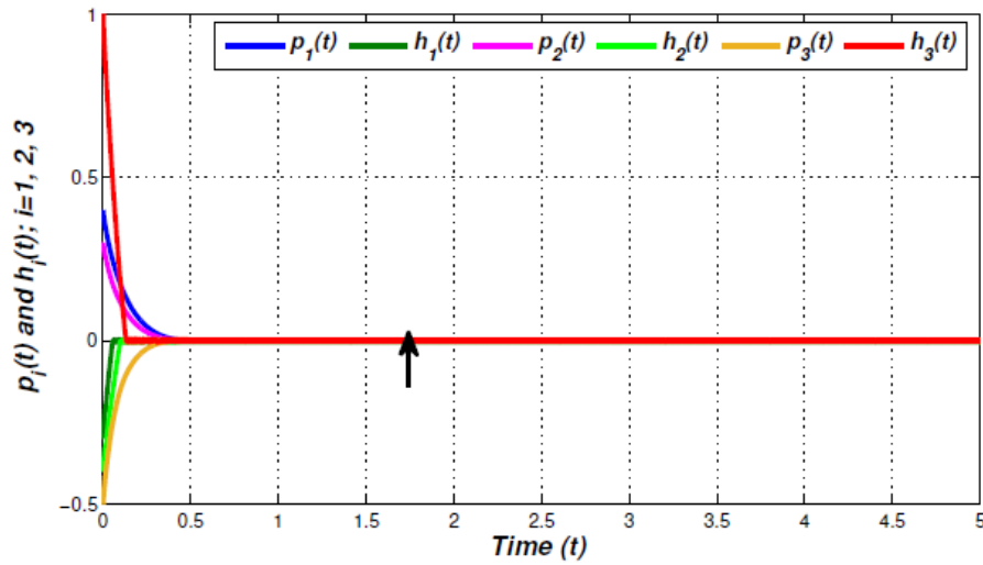
Figure 4 Trajectories state of system (16) under control (12).
