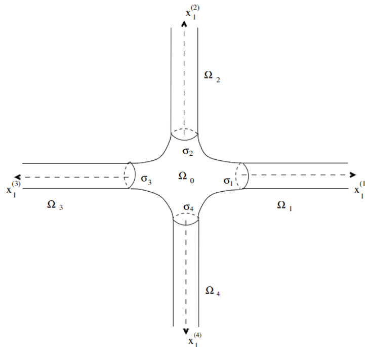
Figure 1 Domain \Omega .
