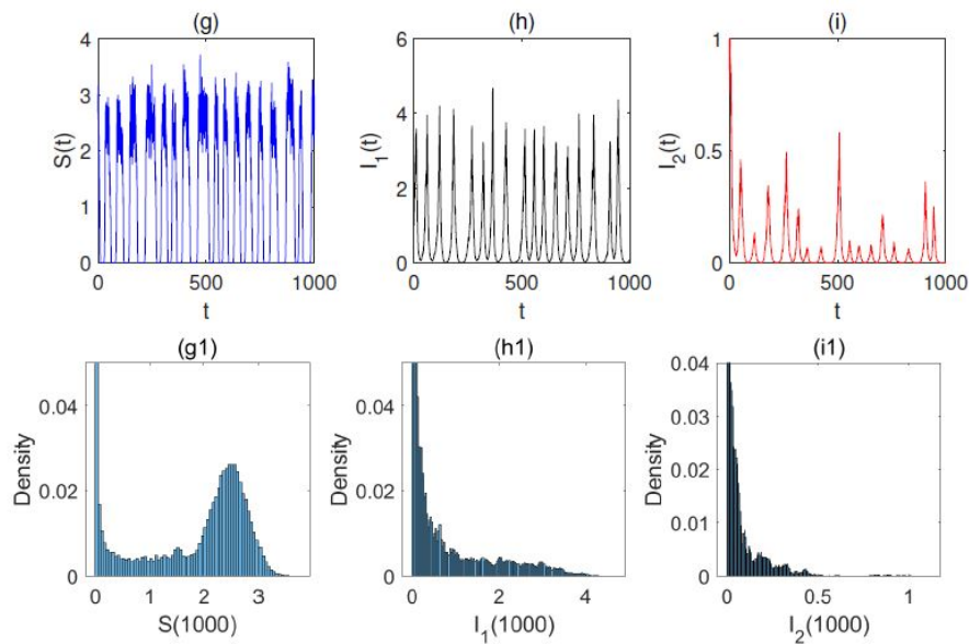
Figure 3 Persistence of I_1(t) and I_2(t) .
