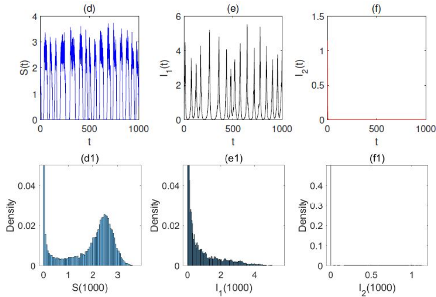
Figure 2 I_1(t) is persistent and I_2(t) is extinct.
