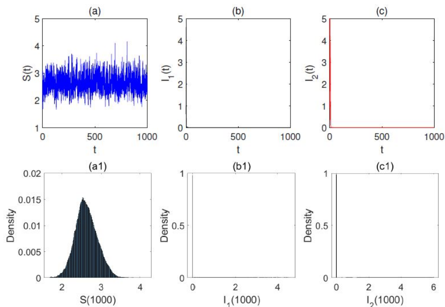
Figure 1 Extinction of I_1(t) and I_2(t)
