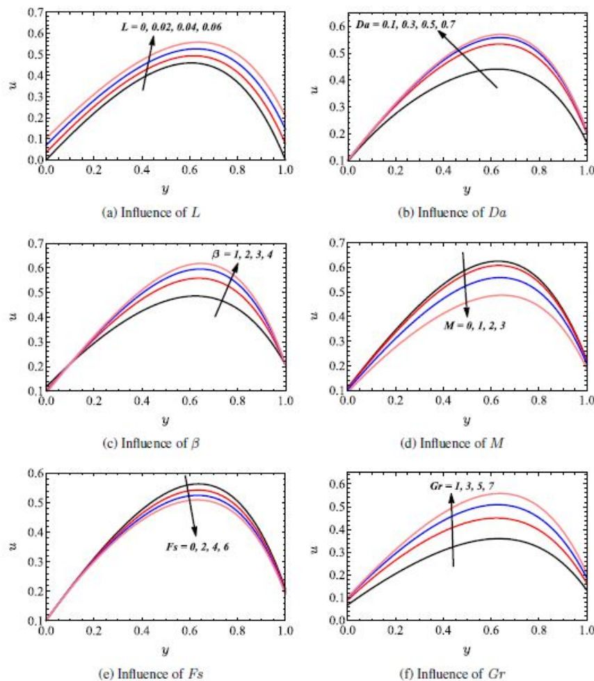
Figure 2. Velocity distributions.
