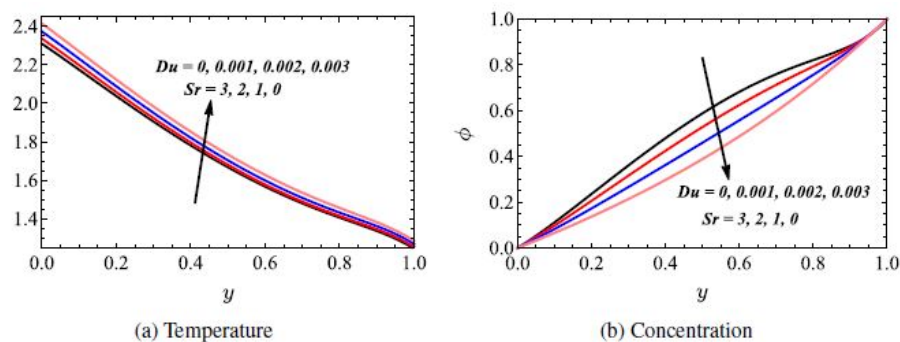
Figure 5. Effect of Du and Sr on the temperature and concentration distributions.
