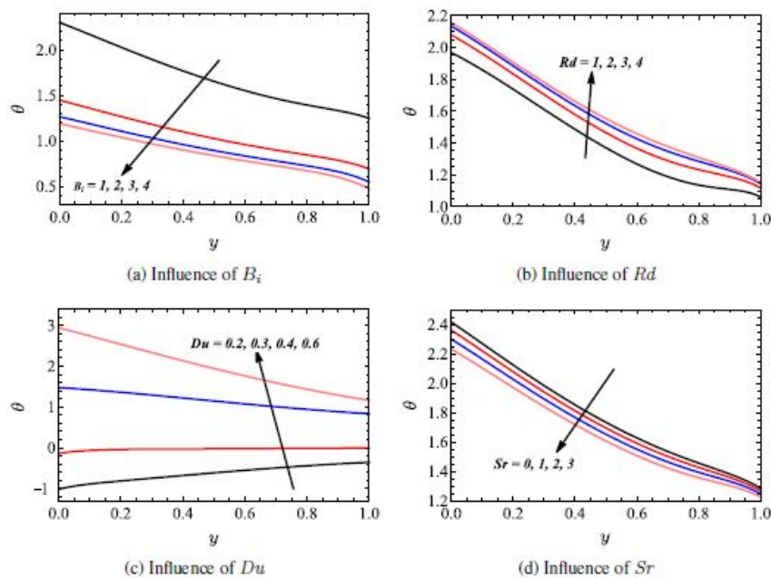
Figure 3. Temperature distributions.
