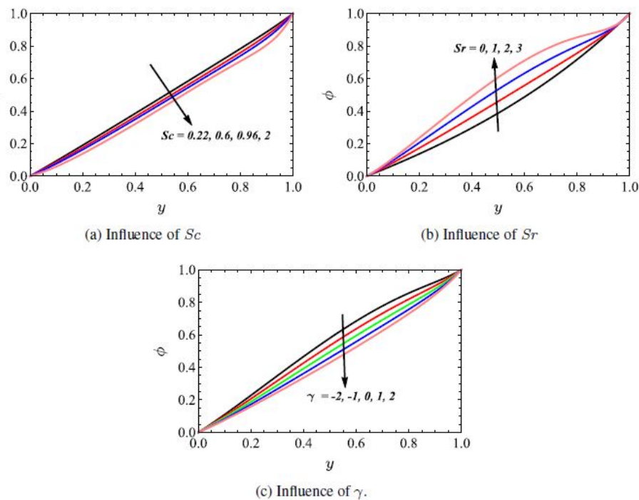
Figure 4. Concentration distributions.
