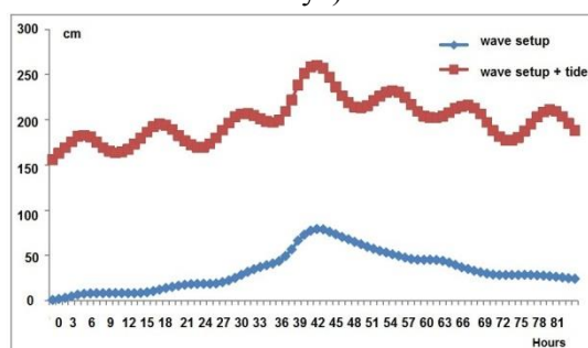
Figure 17. Sea level increase by wave setup, based on WW3 wave output, and by wave setup plus the tide components in Gibara. Forecast from October 23 rd , at 12 UTC (Hurricane “Sandy”).
