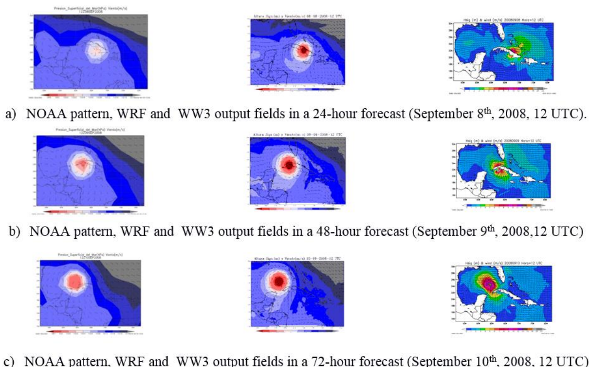
Figure 6. Comparison among NOAA circulation patterns, WRF and WW3 output fields (sea level pressure, wind and wind wave height) in presence of Hurricane "Ike". Forecast from September 7 th , 2008, 12 UTC.
