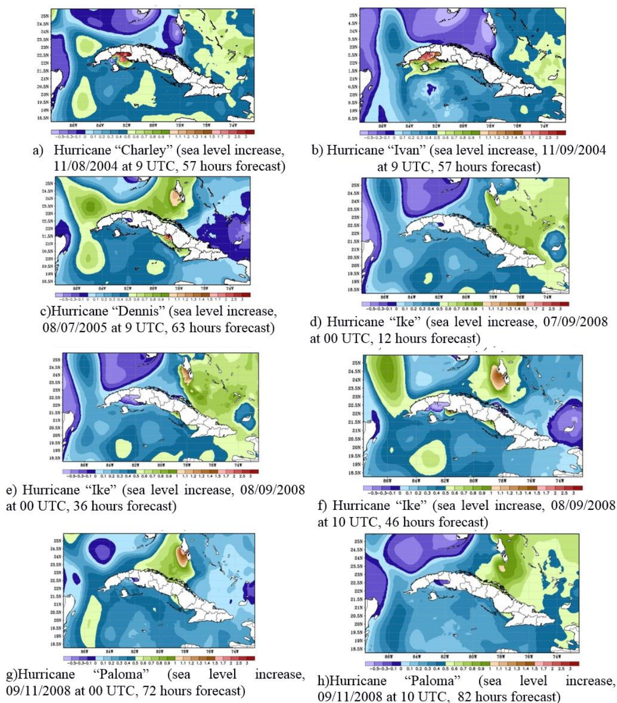
Figure 9. Sea level increase forecast, using ROMS model, in presence of hurricanes “Charley”, “Ivan”, Dennis, “Ike” and “Paloma”
