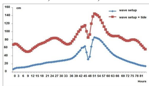
Figure 14. Sea level increase by wave setup (blue line) and by wave setup plus astronomical tide in Havana seafront. Forecast from October 23 rd , 2005 at 00 UTC (“Wilma”)
