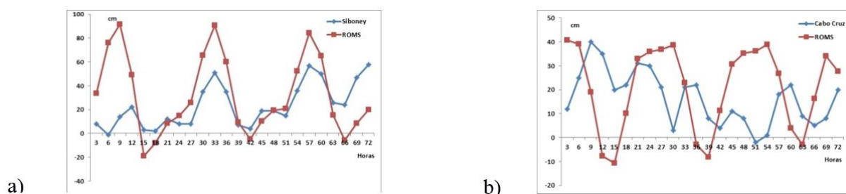
Figure 12. Comparison between tide gauge records of sea level increase and ROMS outputs during a 72-hour forecast in the presence of Hurricane “Dennis”, from July 6 th , 2004, 12 UTC. Locations: a) Siboney b) Cabo Cruz
