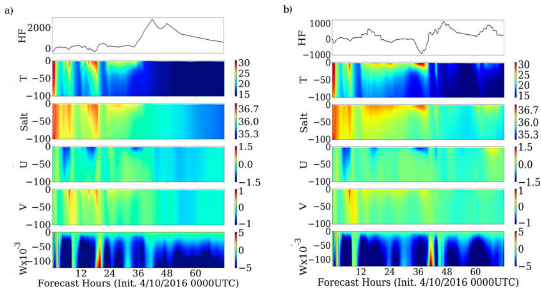
Figure 8. The oceanic dynamics in S2 simulated in (a) ROMS(GFS) and (b) WRF-ROMS experiments; showing Surface net heat flux (HF) in \text{W m}^{-2} , Temperature (T) in ^{\circ}\text{C} , (c) Salinity (Salt) in psu, U,V velocity components in \text{m s}^{-1} and W \times 10^{-3} velocity component in \text{m s}^{-1}
