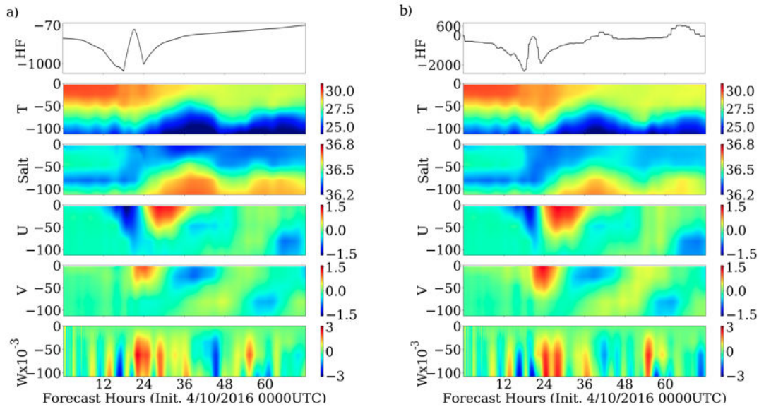
Figure 7. The oceanic dynamics in S1 simulated in (a) ROMS(GFS) and (b) WRF-ROMS experiments; showing Surface net heat flux (HF) in \text{W m}^{-2} , Temperature (T) in ^{\circ}\text{C} , Salinity (Salt) in psu, U and V velocity components in \text{m s}^{-1} and W \times 10^{-3} velocity component in \text{m s}^{-1}
