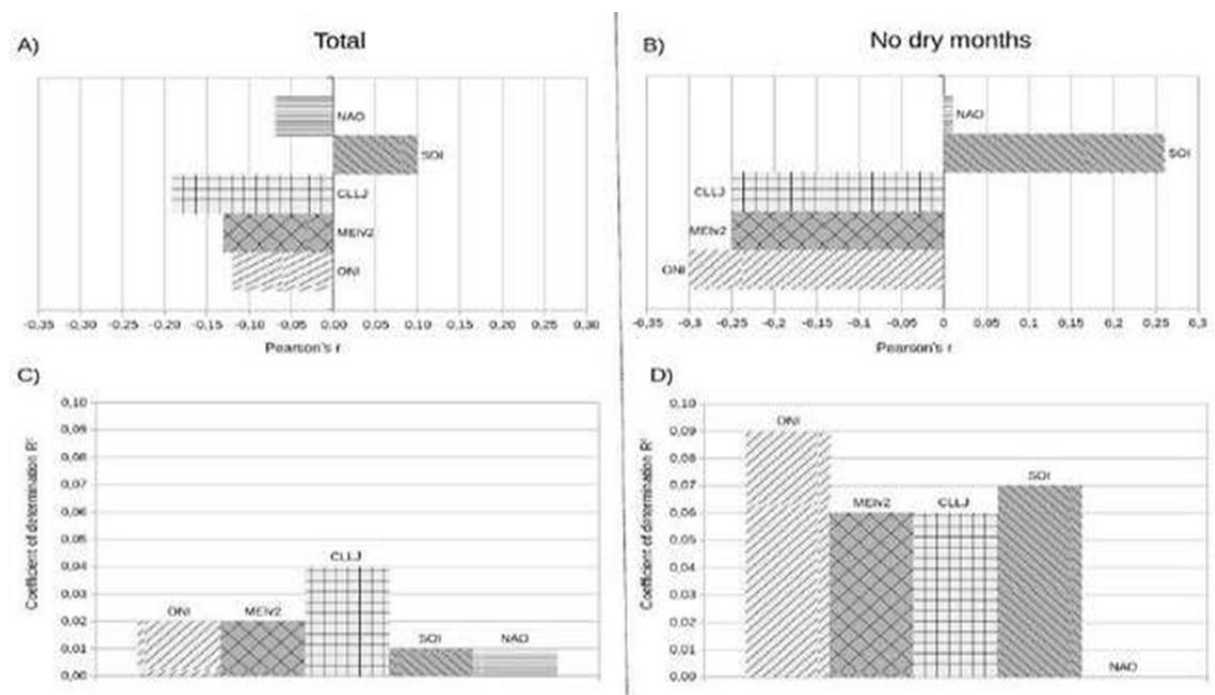
Figure 7. Correlation between precipitation and climate indexes, with and without dry months
