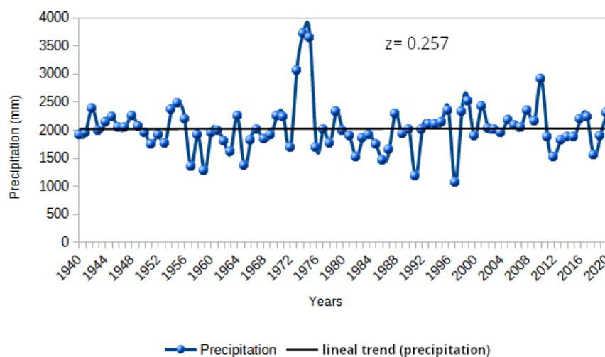
Figura 2. Mann Kendall distribution of interannual rainfall in San Ramon
