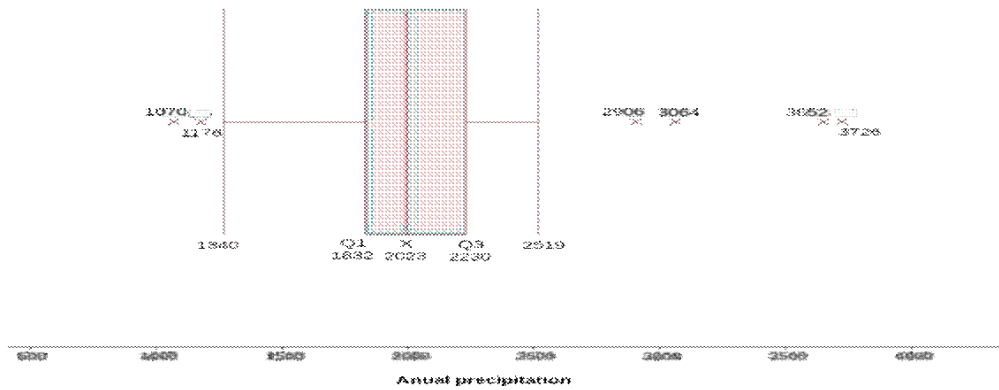
Figure 5. Wisker-box diagram of interannual precipitation, 1940-2020
