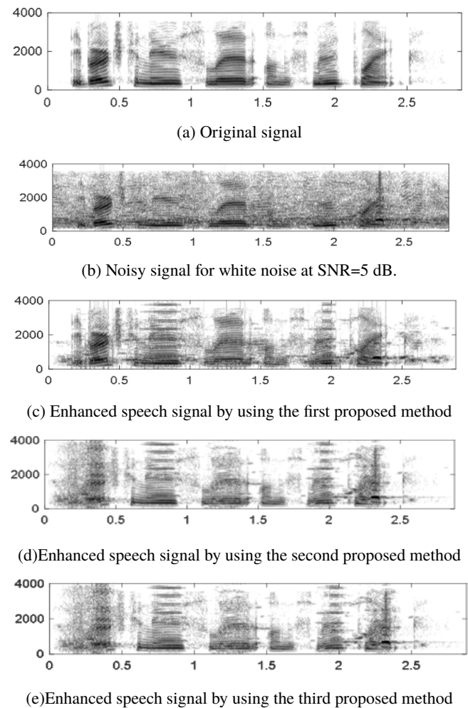
Figure 8: Simulation results for the proposed method in frequency domain.
