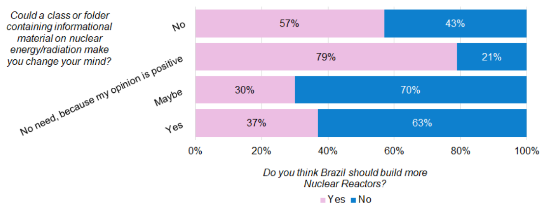
Figure 7: Graph correlating More Reactor X Change Opinion.
