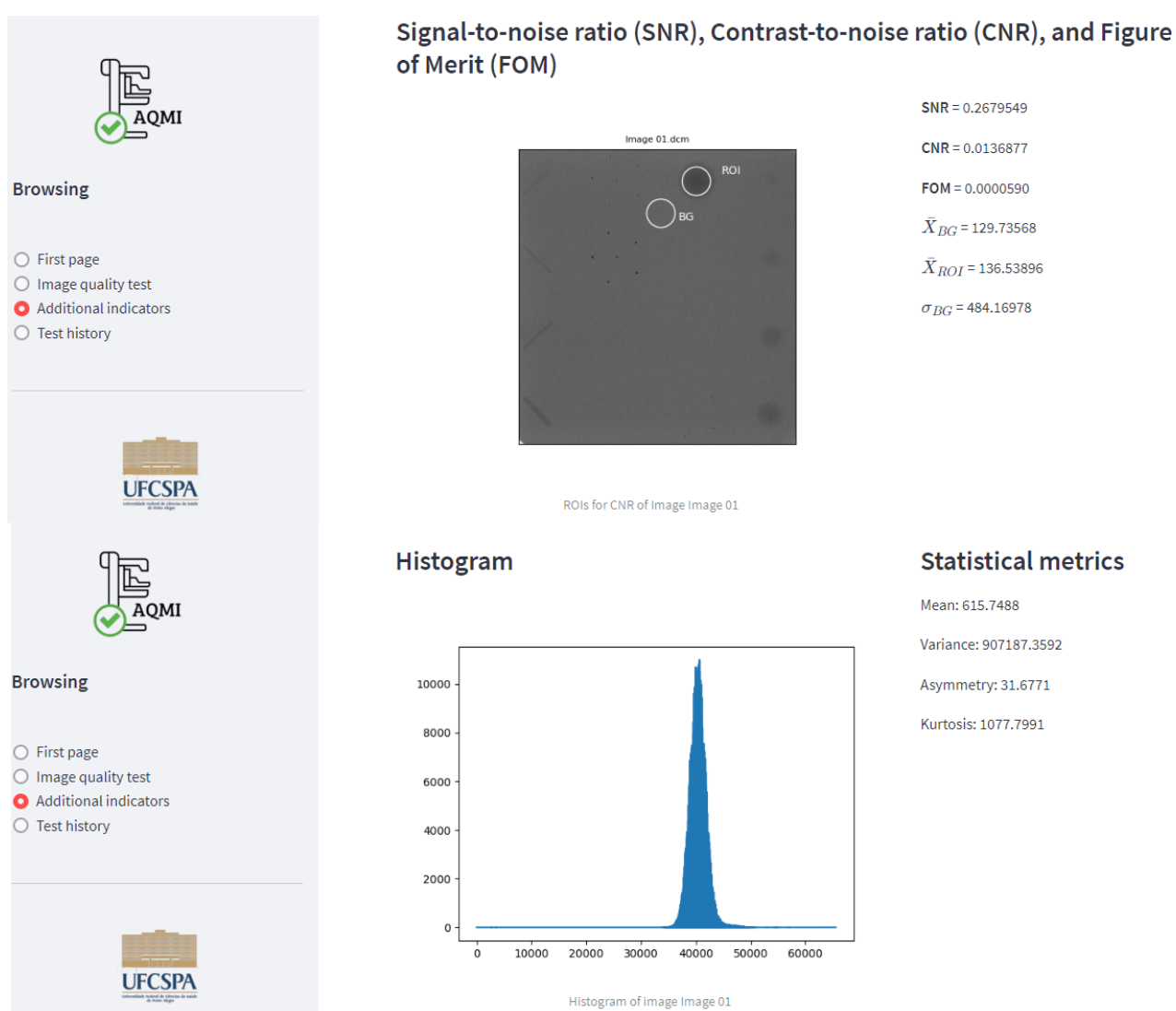
Figure 6 - Layout for the user to visualize the SNR, CNR, FOM and histogram of the assessed image and the statistical metrics of the pixel matrix and the histogram shown in the software interface.
