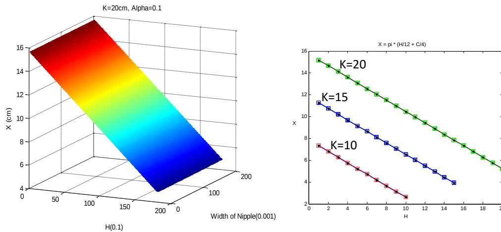
Figure 2. The cube length of X versus cone height of H , a) with the nipple width for K = 20 cm and \alpha = 0.1 , b) the sum of the cone heights for K = 10, 15 , and 20 cm while \alpha and \beta values come near to zero.
