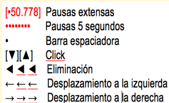
Figure 4: Translog II Linear Representation
