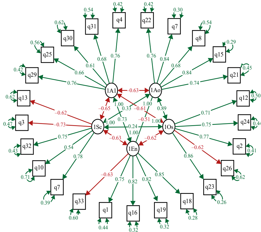
Figure 1. Test data ( n = 434 ) CFA results presented as a graph for TOCA-R adapted. Circle nodes indicate latent variables; square nodes indicate observed indicator variables. Single directed arcs indicate factor loadings, and bidirectional arcs indicate covariance (between different nodes) or error variance (in a single node).
