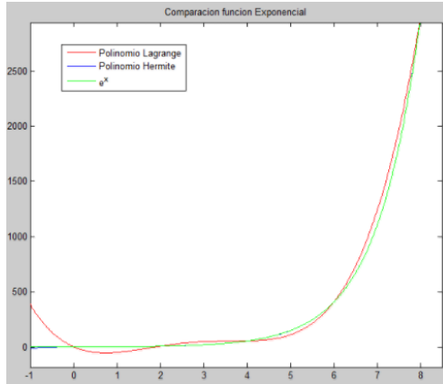
Fig 1. Exponential function
