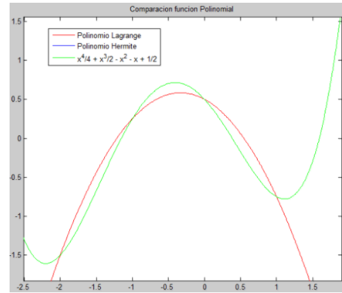
Fig. .3 Graph of the polynomial function
