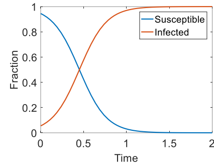
(b) k = 15
