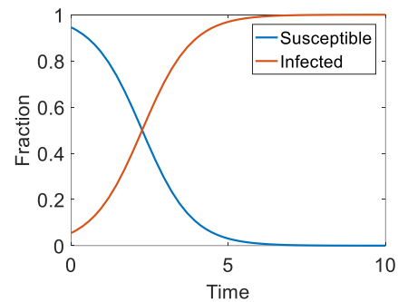
(a) k = 3
