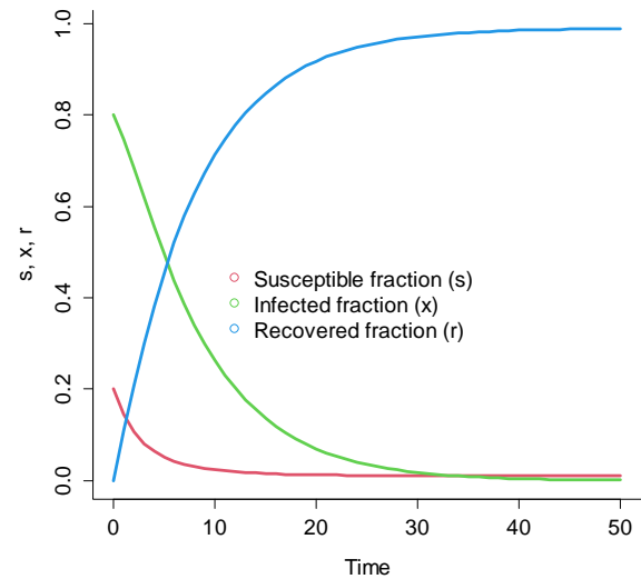
(a) s_0 = 0.2
