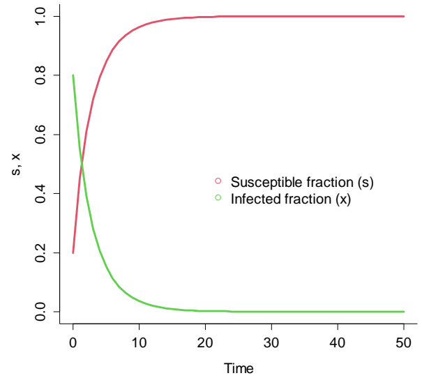
Fig. 7. Computer solution of (10).
