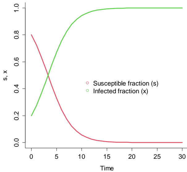
Fig. 2. Dynamics of (2) with \beta = 0.42 and x_0 = 0.2 .
