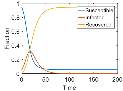
(b) k = 15
