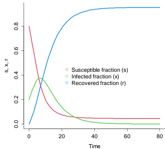
(b) s_0 = 0.8
