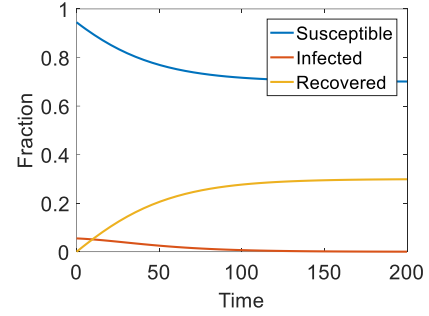
(a) k = 5
