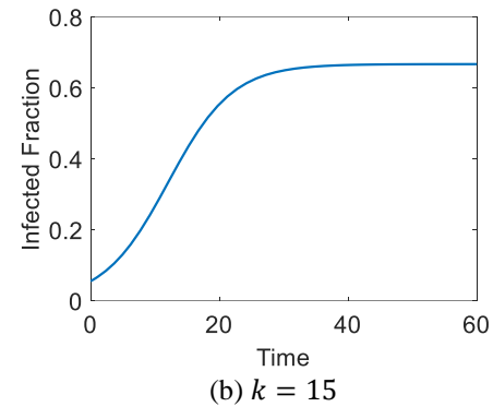
Fig. 11. Fraction of infected nodes for a network k -regulate with x_i(0) = 0.055 in all cases, \beta = 0.02 , \gamma = 0.1 y n = 10^5 nodes.
