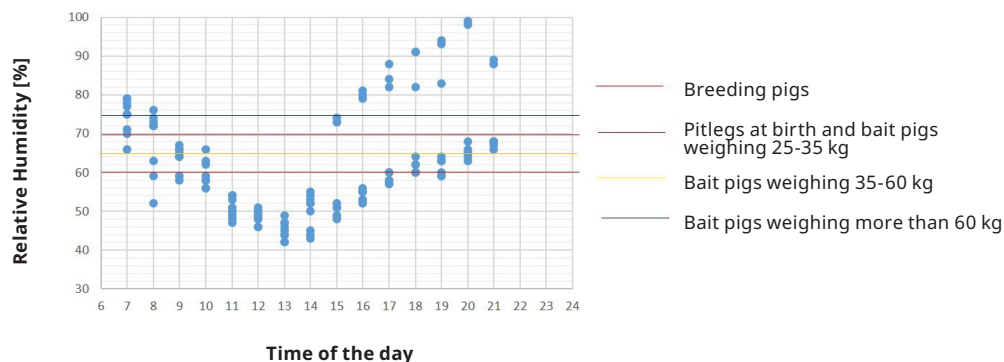
Fig. 4. RH behavior inside Pigpen no. 2.
