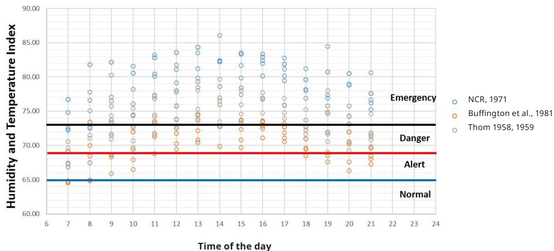
Fig. 5. HTI behavior inside Pigpen no. 1.
